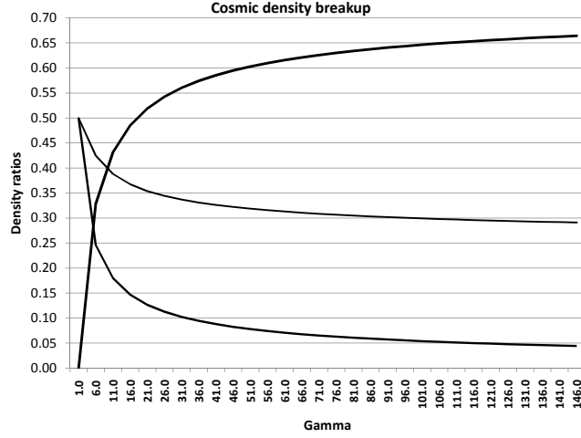
Fig. 1. Past, present and future cosmic density breakup
