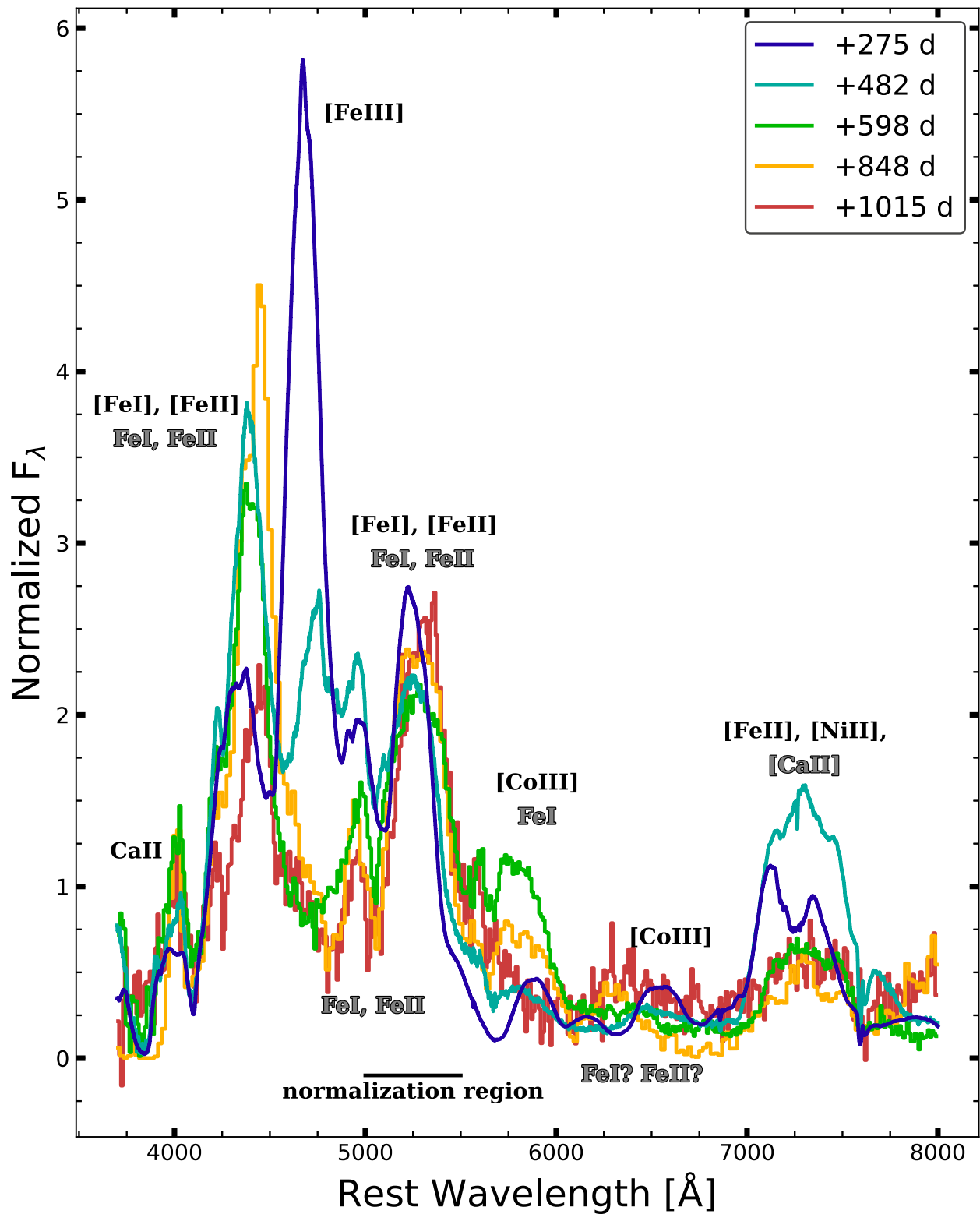
Figure 2. Spectroscopic comparison at various epochs using the same color scheme as Figure 1 but normalized by the mean flux near 5300 Å. Dominant line identifications before and after the distinct ionization transition at ~500 days are given in black and gray, respectively. Lines with a “?” indicate that the line’s contribution to the observed spectral feature is unclear. Fe emission lines after the ionization transition are likely blends of forbidden and permitted transitions (Fransson & Jerkstrand 2015), but we omit the bracket notation for visual clarity.
