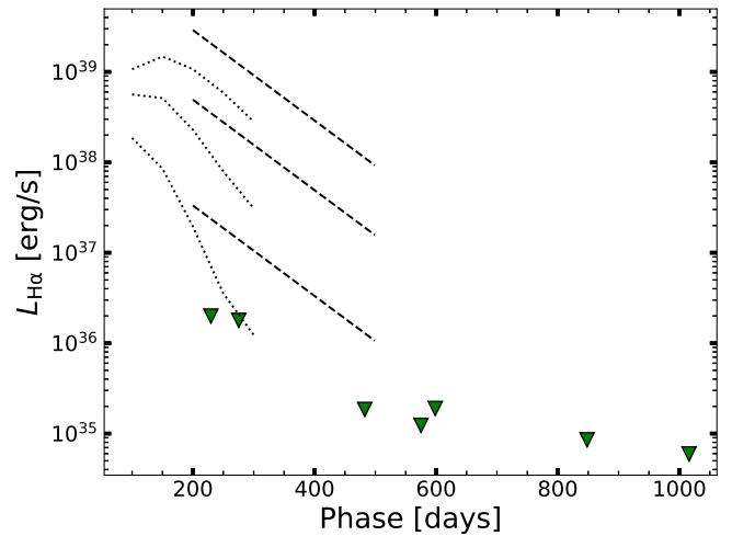
Figure 6. Nondetections of H\alpha (inverted triangles) compared to the models of Dessart et al. (2020, dotted lines, 100 days \lesssim t_{\text{max}} \lesssim 300 days) and Botyánszki et al. (2018, dashed lines, 200 days \lesssim t_{\text{max}} \lesssim 500 days) for ablated masses of (10^{-1}, 10^{-2}, 10^{-3}) M_{\odot} , from top to bottom. Flux limits for H\alpha , He I \lambda 5876 , and [O I] \lambda 6300 are provided as data behind the figure.
