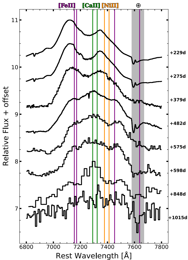
Figure 3. Temporal evolution of the 7300 Å feature, transitioning from [Fe II] + [Ni II] to [Ca II] around \sim 480 days after t_{\max} (see Section 3.2).
