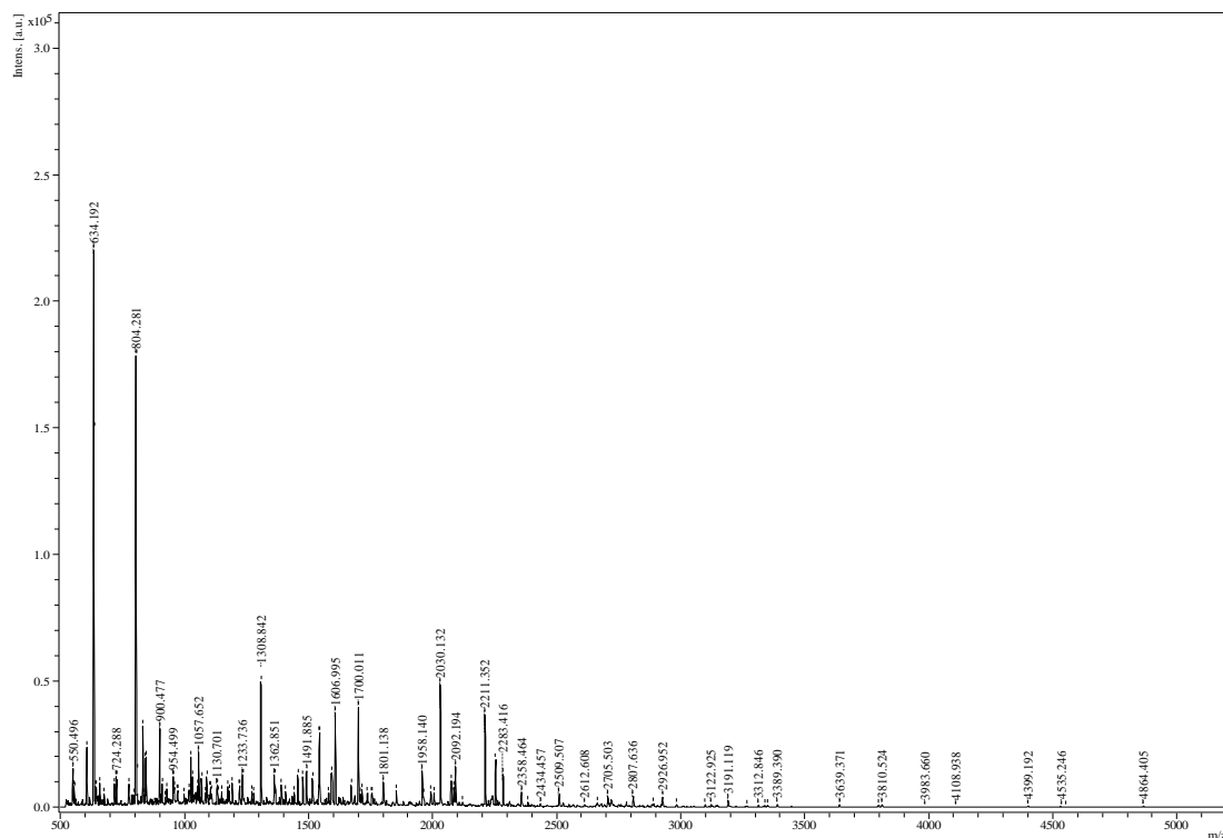
Fig. 3. MALDI-TOF/MS results
