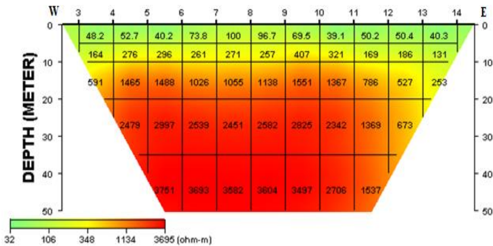
Fig. 8. 2D inverted resistivity sections beneath Traverses 6
