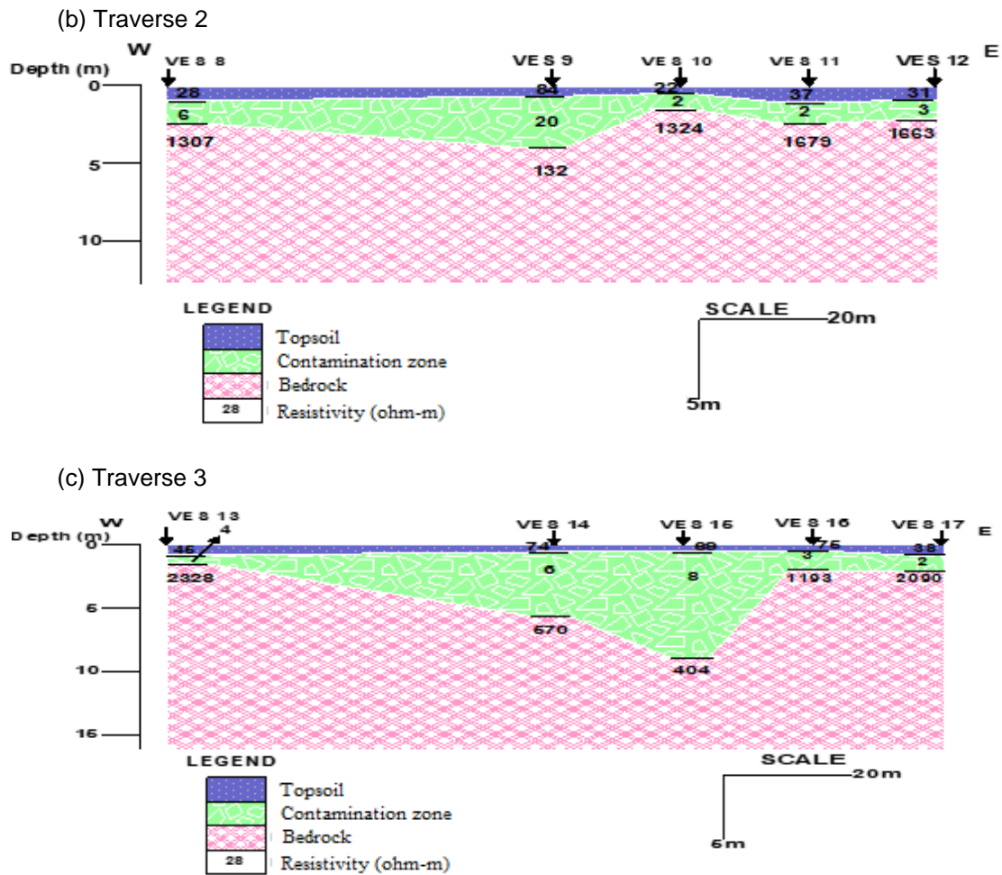
Fig. 4(a-c). Goelectric section beneath Traverses 1- 3 in the study area
