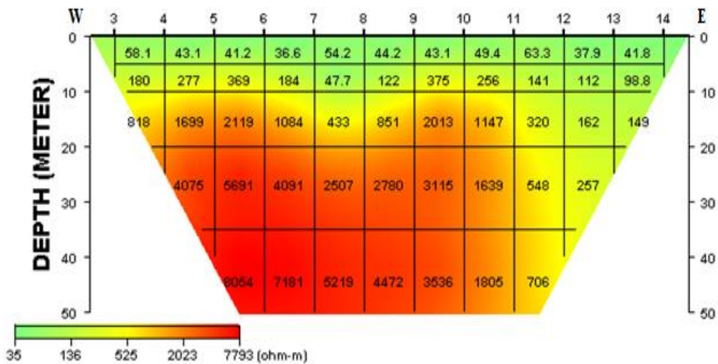
Fig. 6(a-d). 2D inverted resistivity section beneath Traverses 1-4
