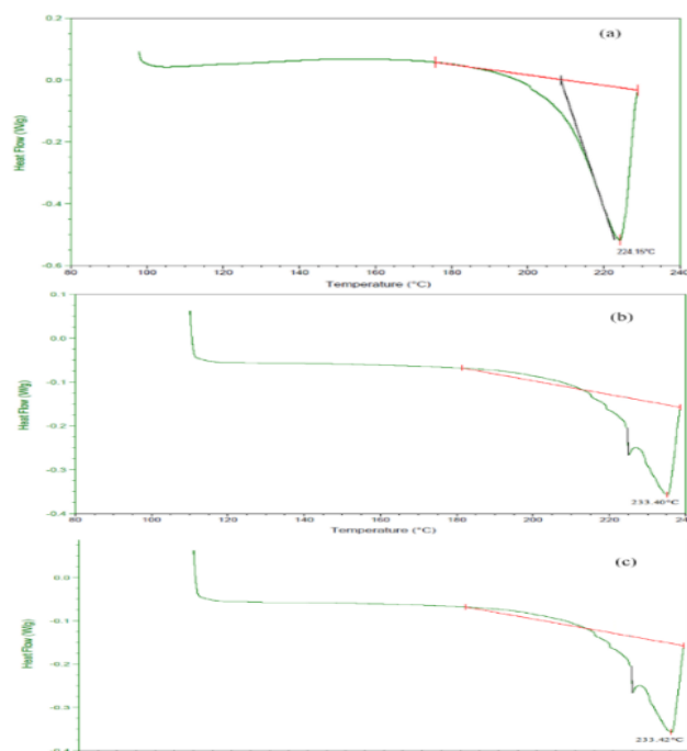
Fig. 6. DSC thermogram of SMZ, (a), Physical mixture of drug and poloxamer 407 (b), SDSMFF8 (c)
