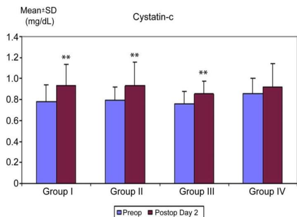
Fig. 3. Cystatin-C level
