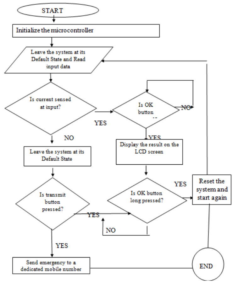
Fig. 5. Algorithm chart of device
