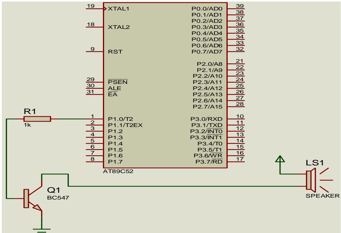
Fig. 3. The alarm unit
