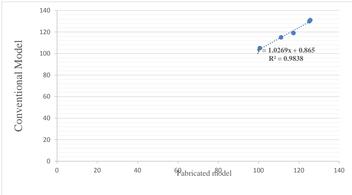
Fig. 7. Correlation model of fabricated model result (mg/dl) against standard model result(mg/dl)
