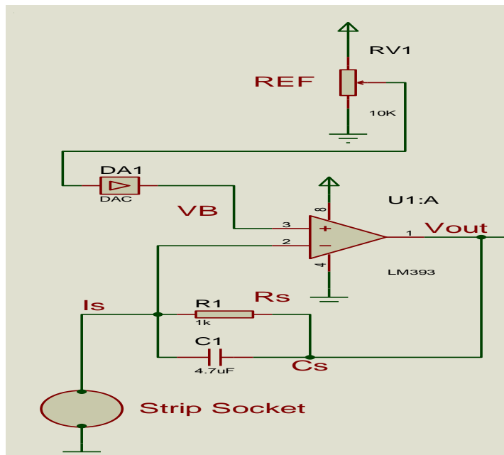
Fig. 2. Glucose level input signal converter
