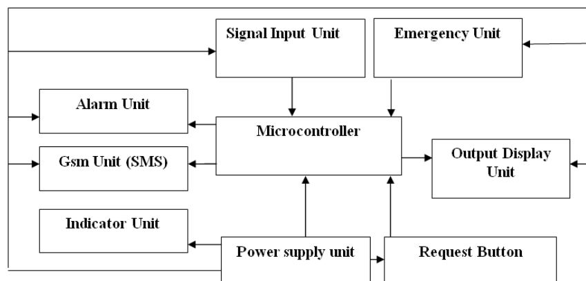
Fig. 1. Block diagram of the glucometer
