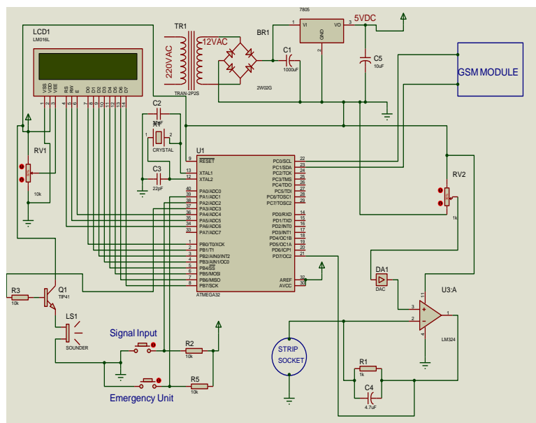
Fig. 6. Circuit diagram of the Glucometer with GSM module
