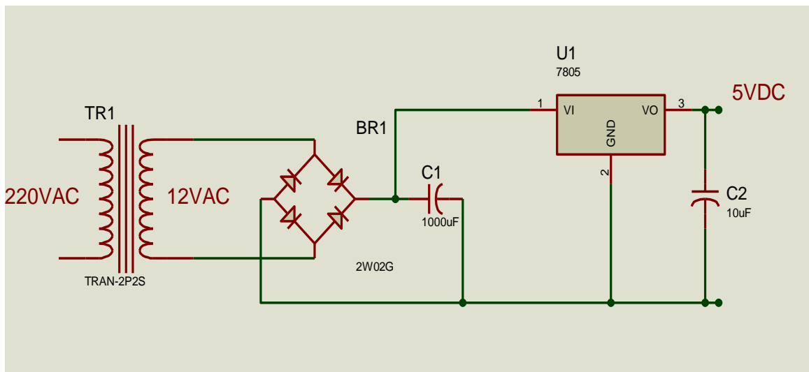
Fig. 4. The power supply unit
