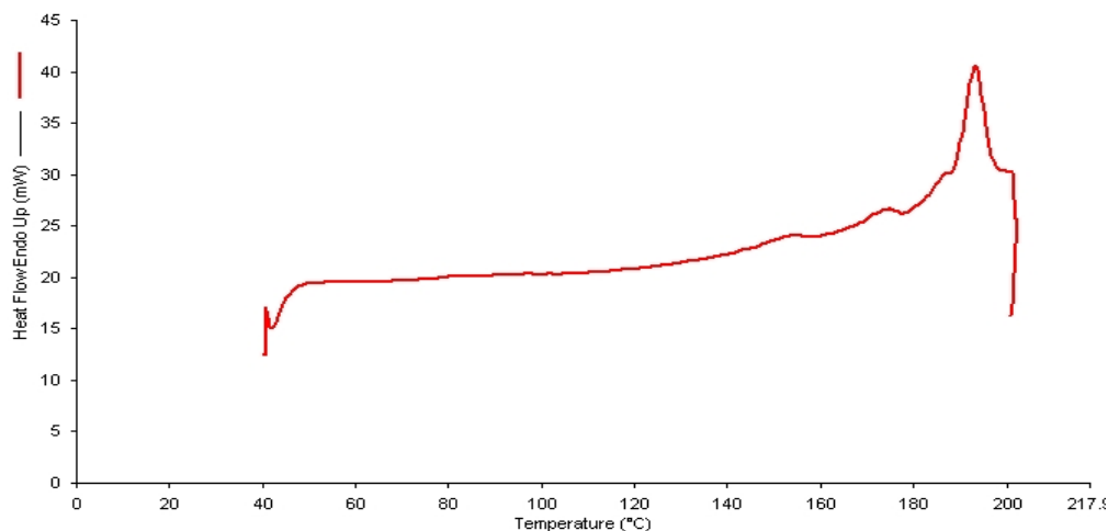
Fig. 2. DSC thermal analysis for carbamazepine total mixture
