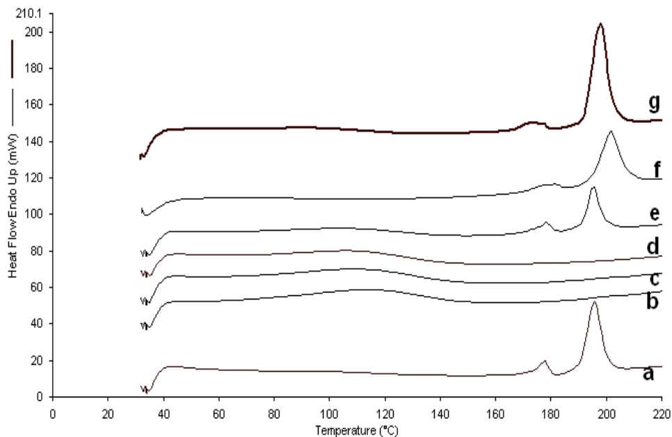
Fig. 1. DSC thermal analysis for : a- carbamazepine alone, b- HPMC K 100 LV, c- HPMC , d-HPMC K 15M, e- carbamazepine/ HPMC K 100 LV 1:1 physical mixture, f- carbamazepine /HPMC 1:1 physical mixture, g- carbamazepine /HPMC K 15M 1:1 physical mixture
